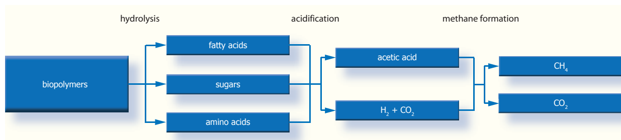
Figure 5.3 – Schematic depiction of the degradation steps with sludge digestion
