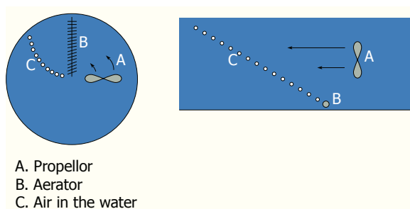
Figure 3.17 – Aeration combined with horizontal flow, stirred up by a propeller (Rotoflow).
