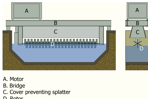
Figure 3.12 - Aeration rotor (Passavant)
