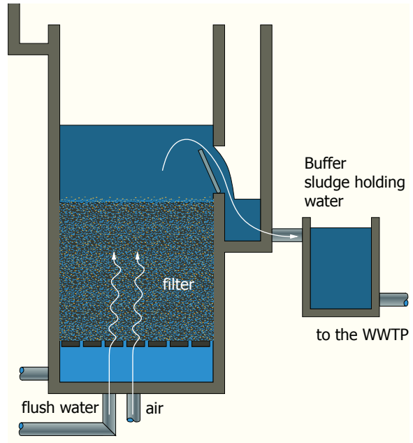
quick-run filter during flushing
