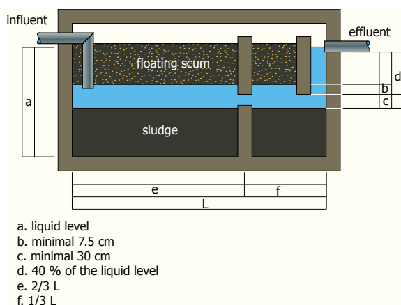
Figure 5.5 - Septic tank
