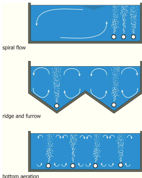
Figure 3.13 - distribution of the elements over the bottom creates spiral flows (whirlpools); a. spiral flow; b. ridge and furrow; c. bottom aeration
