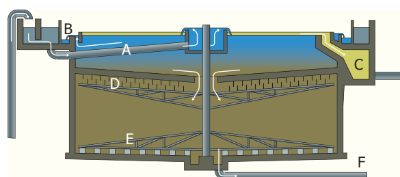
Figure 5.6 - Imhoff tank
