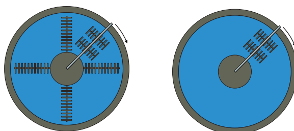
Figure 3.16 – aeration combined with horizontal flow, stirred up by a rotating bridge (Schreiber).
